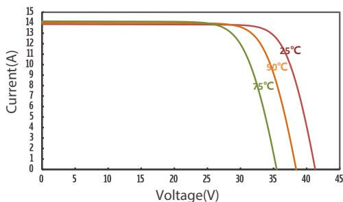
IV Curves of JT450SHh at different Temp
