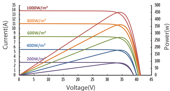
IV Curves of JT450SHh at different irradiances
