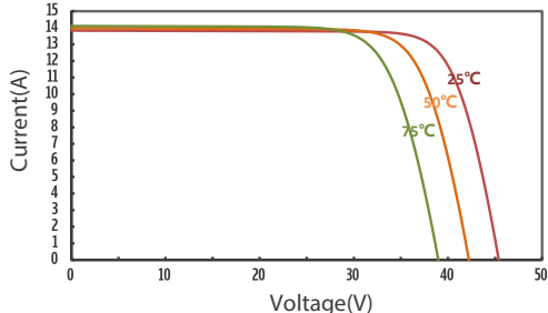
IV Curves of JT495SLh(B) at different Temp
