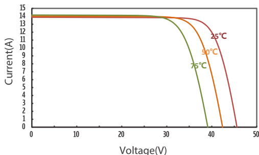
IV Curves of JT500SFh at different Temp
