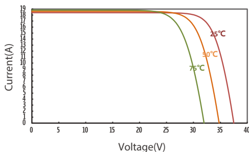
IV Curves of JT550SWk at different Temp
